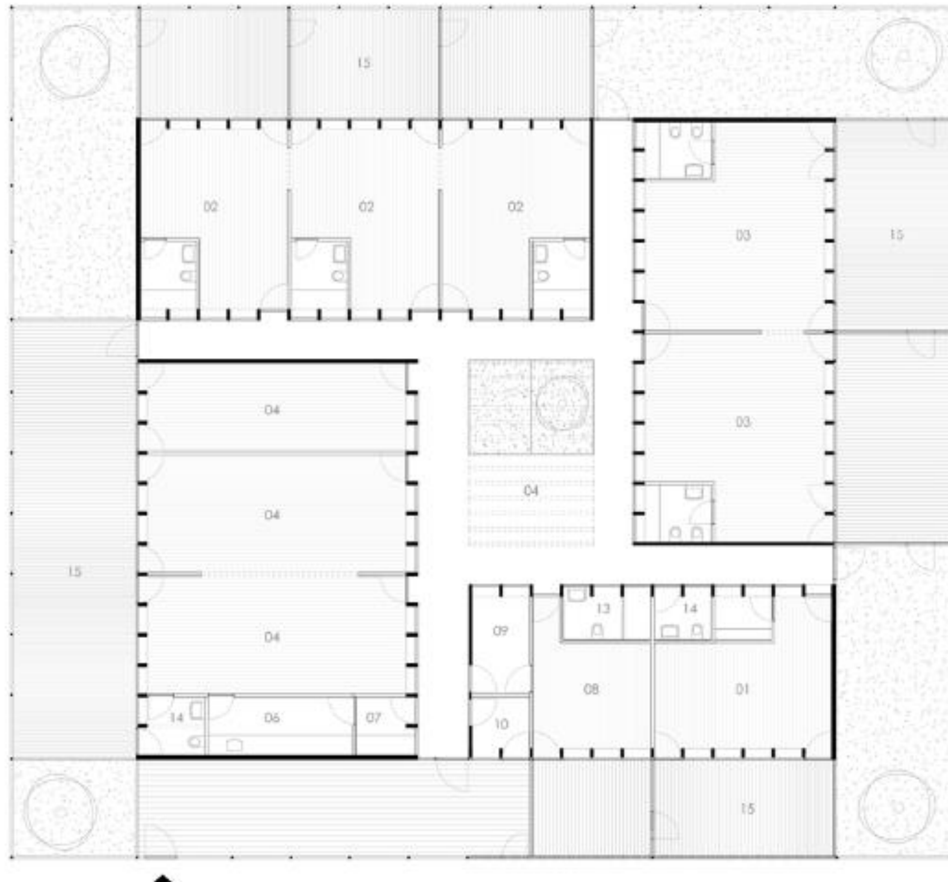
Ground Floor
